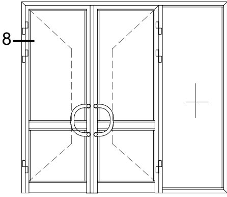
DIŐA AÇILIR BİNİLİ KAPI DETAY OUTWARD OPENING OVERLAPPING DOOR DETAIL
