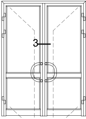
İÇE AÇILIR ADAPTÖRLÜ BİNİLİ KAPI DETAY INWARD OPENING OVERLAPPING DOOR DETAIL
