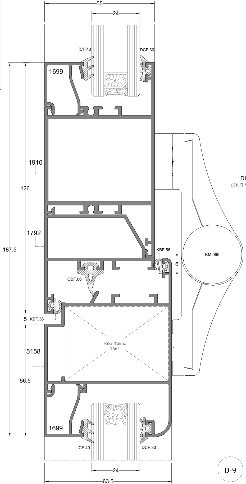
DIŞA AÇILIR BİNİLİ KAPI DETAY OUTWARD OPENING OVERLAPPING DOOR DETAIL
