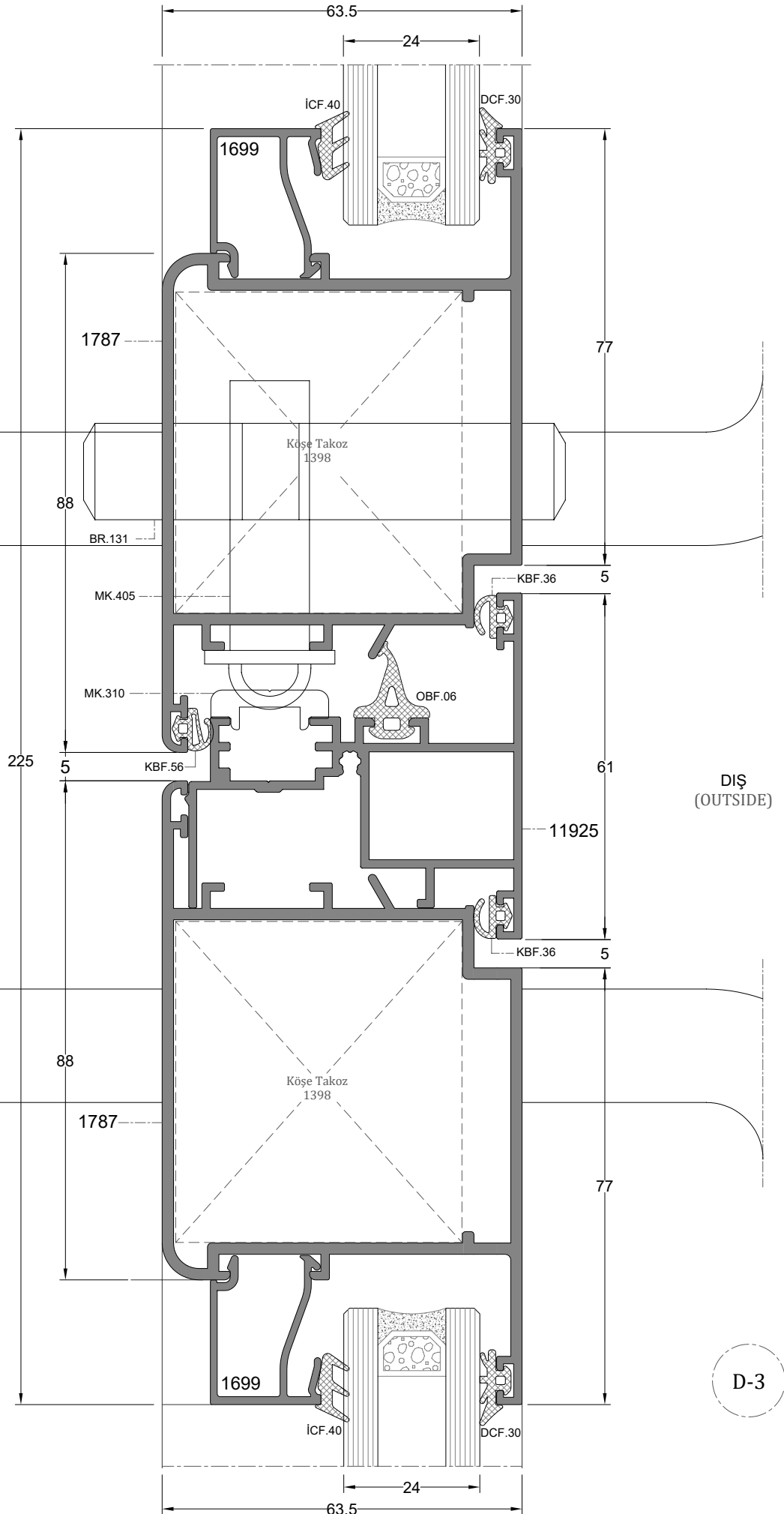
İÇE AÇILIR ADAPTÖRLÜ BİNİLİ KAPI DETAY INWARD OPENING OVERLAPPING DOOR DETAIL
