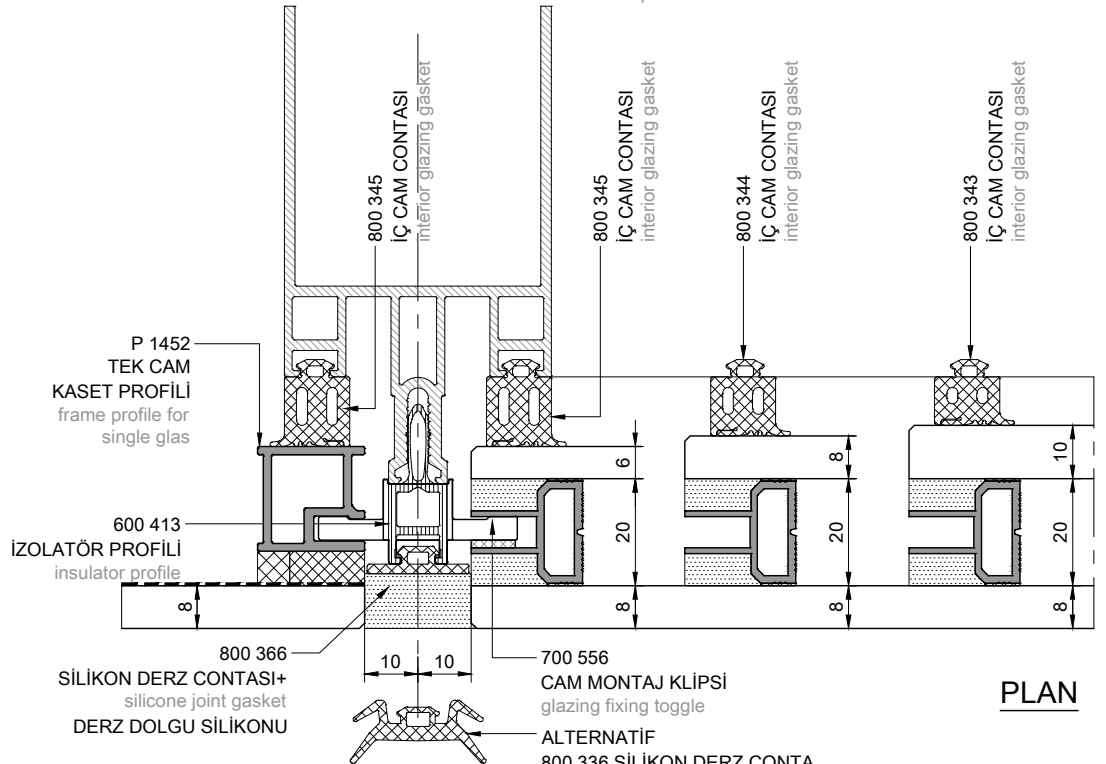
700 556 CAM MONTAJ KLİPSİ glazing fixing toggle
